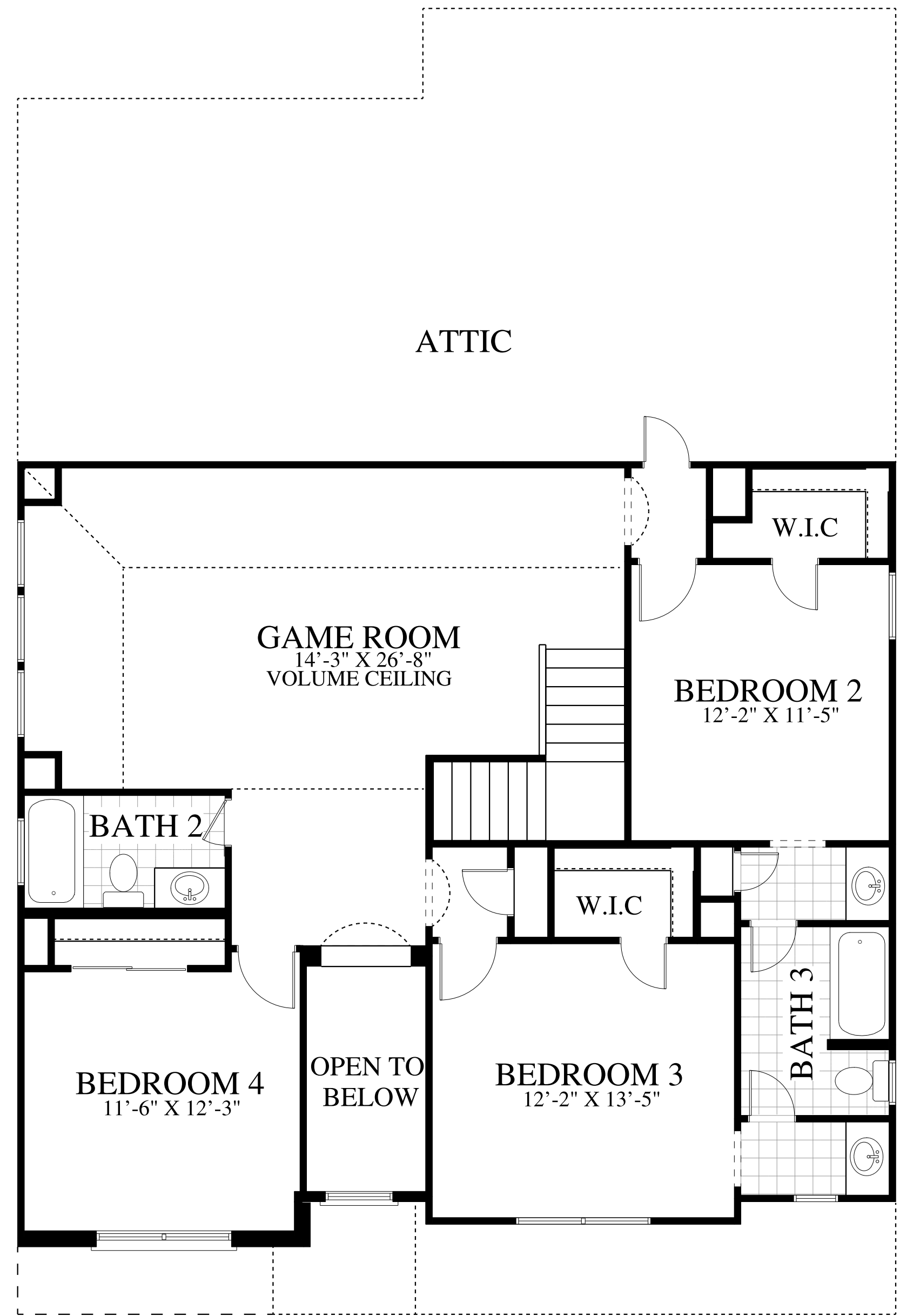
SECOND FLOOR PLAN A, B & C 1214 S.F.
