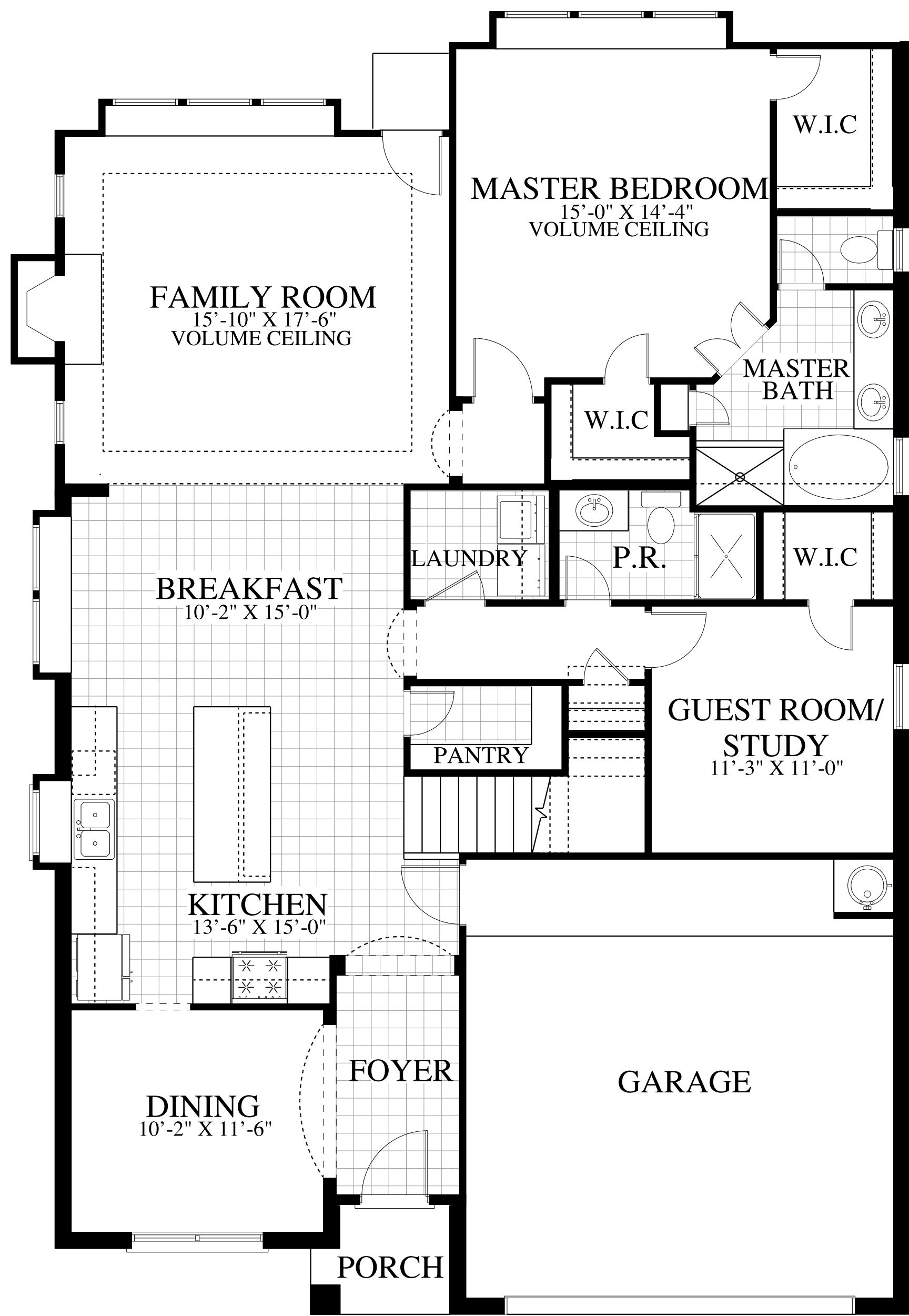
FIRST FLOOR PLAN A & B 1702 S.F.
