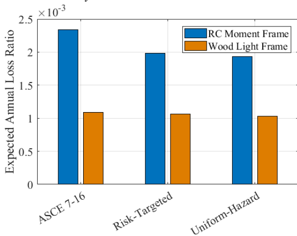
Figure 10 - Comparison of EAL ratio (EAL normalized by the replacement value of the building) among seismic design maps for wood light frame and RC moment frame buildings in San Jose, CA.
