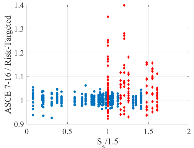
Figure 5 - Ratio of EAL from ASCE 7-16 (ASCE, 2016) seismic design maps to the EAL from a risk-targeted seismic design map vs. the short period spectral acceleration normalized by the minimum deterministic value. Sites where design is governed by deterministic caps in ASCE 7-16 are shown in red.
