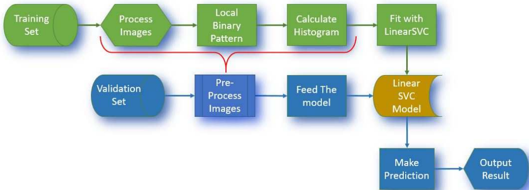
Fig. 5. Binary Classification
