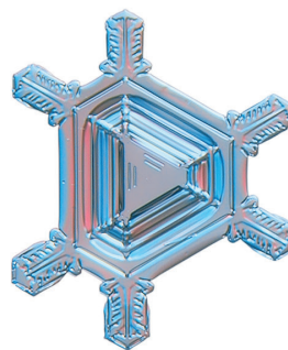
Triangular Crystals
