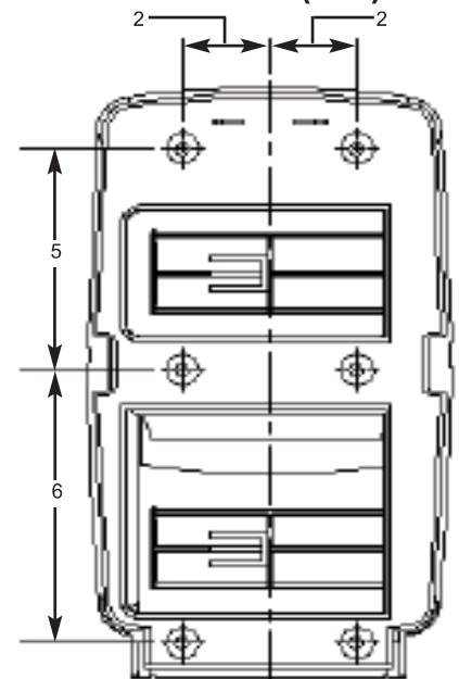
Back (mm)
