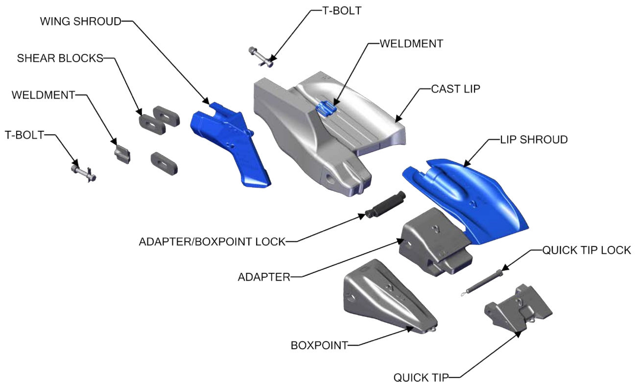
FIGURE 1. Cast lip and G.E.T. labels
