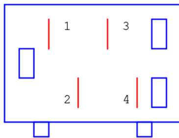
J1 Pin Positions Plug Backside
