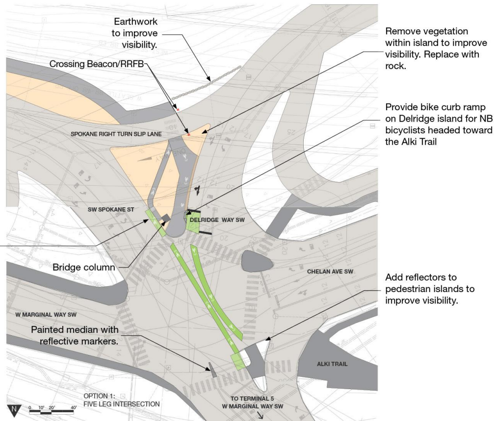
Figure 4: Enhanced At-Grade Crossing (Short Term)
