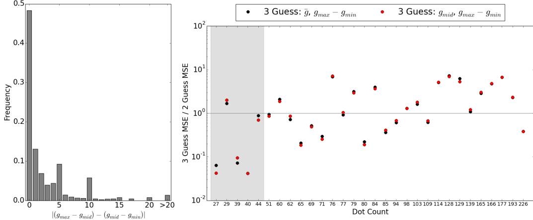
Figure 4: Experimental results for 3-guess responses. Left: symmetry of gaps in 3-guess triplets. Right: ratios of the mean squared error (MSE) for bootstrapped population of differently configured 3-guess weighted median estimators, compared to a 2-guess MSE. The 3-guess MSE does not vary much between different estimator configurations, and is not clearly better or worse than the 2-guess MSE. The shaded region indicates dot counts where an “integer constraint” effect is suspected, see text.
