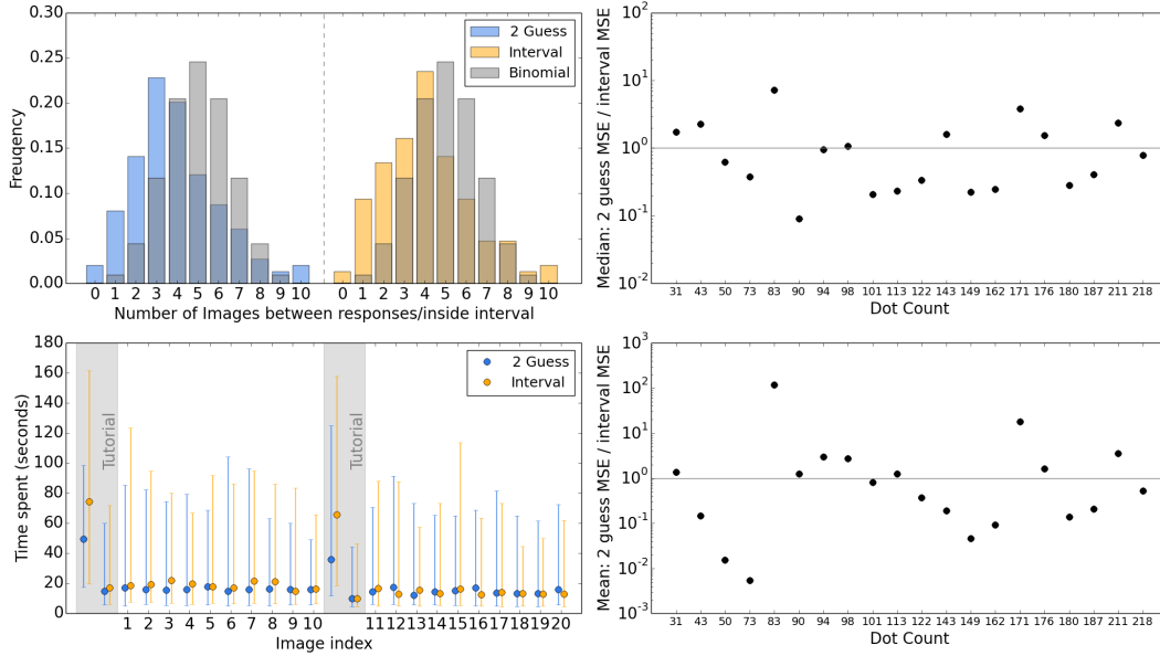
Figure 5: Results for interval vs. 2-guess comparison. Top left: frequency with which the true dot count was inside/between intervals/guesses. Bottom left: time taken to play the game. Half the users played the interval game, then the 2 guesses game; the other half played the 2 guesses game, then the interval game. Circles indicate medians and error bars are empirical 5th/95th percentiles of the population. Right: ratios of MSE for bootstrapped populations of 2-guess and interval weighted median (top) and weighted mean (bottom) estimators. Ratios below 1.0 indicate the 2-guess-weighted MSE is lower than the interval-weighted MSE.
