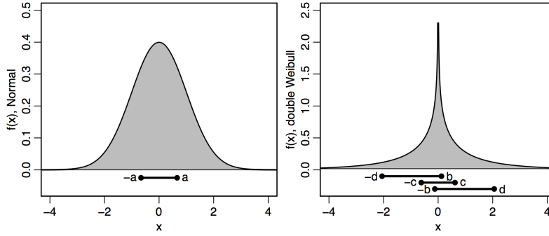
Figure 1: Left: for the two guesses scoring rule, the unique optimal response set for a zero-mean Normal distribution is \{-0.674\sigma, 0.674\sigma\} . Right: as an example of how even symmetric and unimodal non-log-concave distributions may not have a unique optima, for the zero-mean double Weibull distribution [Mease et al., 2004] there are two asymmetric optima \{-d, b\} and \{-b, d\} that both outperform the best symmetric answer \{-c, c\} .
