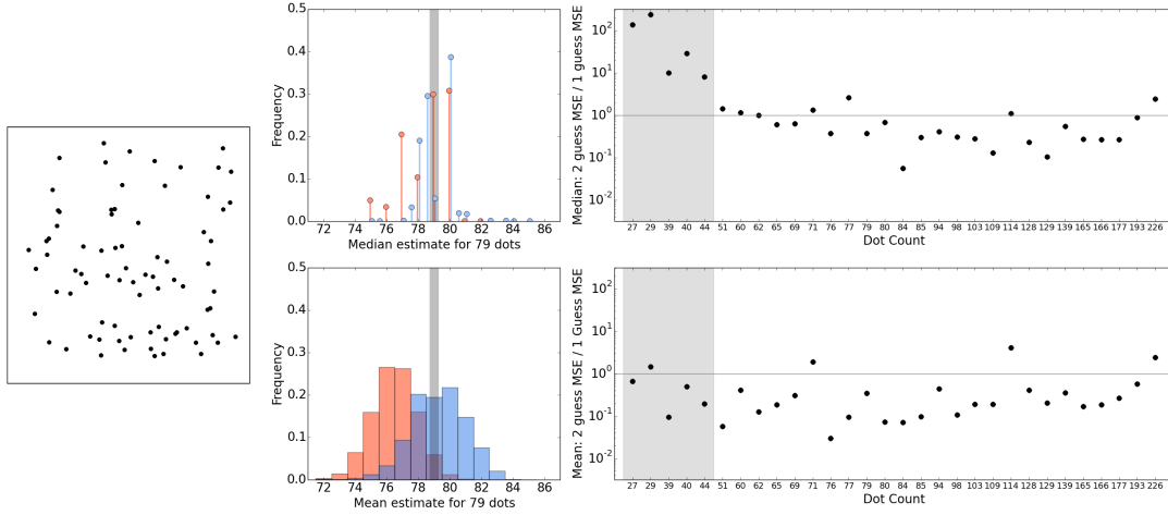
Figure 3: Experimental results for 1- and 2-guess responses. Left: an image from the game, with 79 dots. Center: bootstrapped distributions of mean and median estimators for the 1-guess (red) and weighted 2-guess (blue) responses for the 79 dot image. Right: ratios of mean squared error (MSE) for bootstrapped population of median and mean estimators. The shaded region indicates dot counts where an “integer constraint” had a pronounced effect, see text. Ratios below 1.0 indicate the weighted 2-guess MSE is lower than the unweighted 1-guess MSE.
