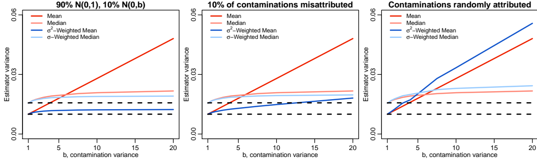
Figure 2: Estimators variance for contamination models with 100 samples. Left: a contaminated Normal distribution. Center and Right: the same contamination model with partially misattributed weights. Dashed lines indicate variance under uniform certainty.
